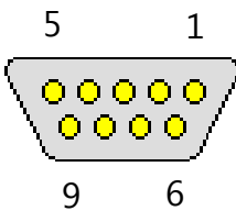
Wiring Harness Connector as viewed from REAR (wired side)
