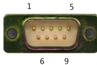
Front of Connector B
