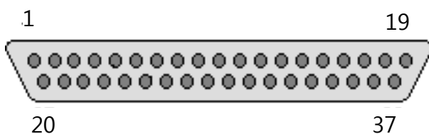
Wiring Harness Connector as viewed from REAR (wired side)
