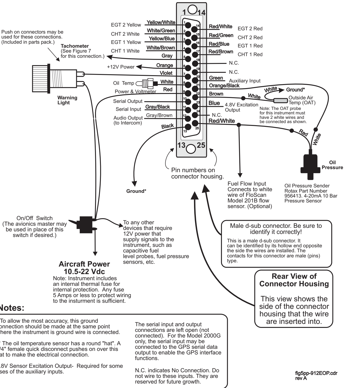
Figure 5 -- Connector A Wiring - Model 2000 for Rotax 912 engines with electronic Oil Pressure sensor - (Ext CJ)
