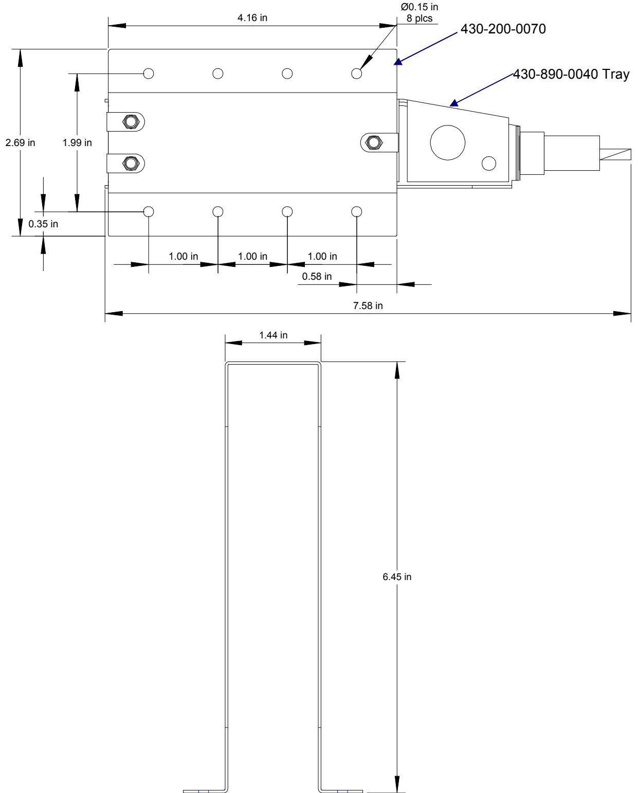
Figure 5-2 PDA360XR vertical Mounting Option (not to scale)
