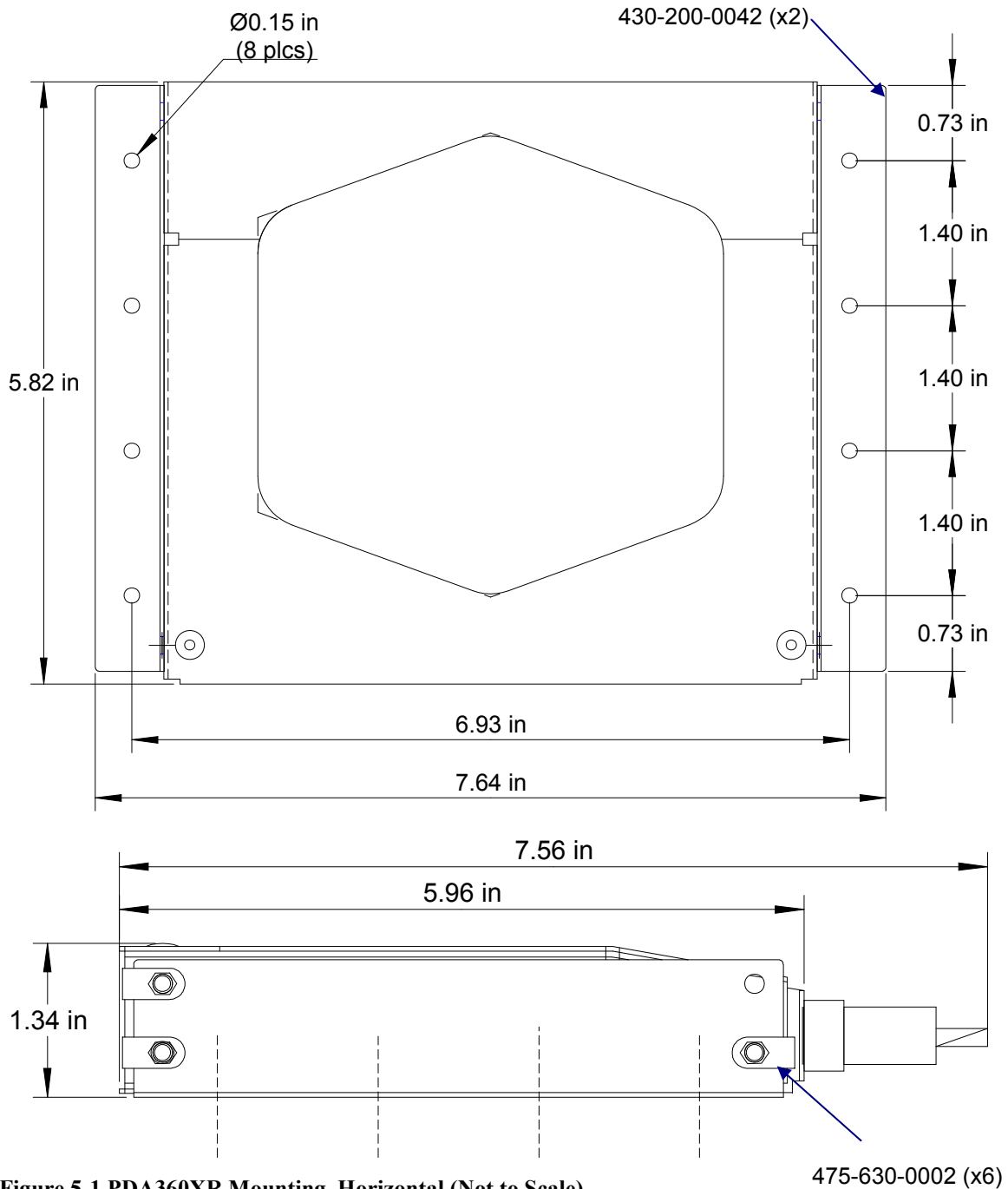
Figure 5-1 PDA360XR Mounting, Horizontal (Not to Scale)
